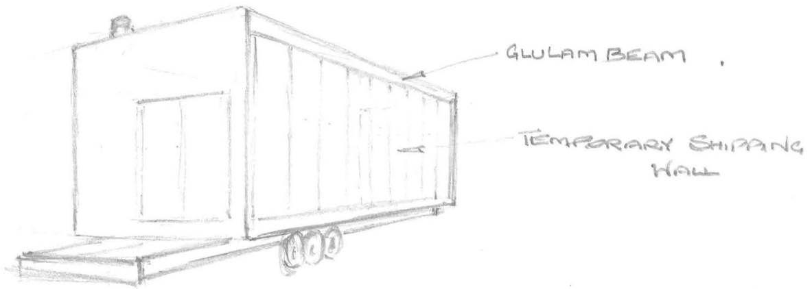
EXISTING UNIT: 10' WIDE, 36' LONG, 9' CEILING
